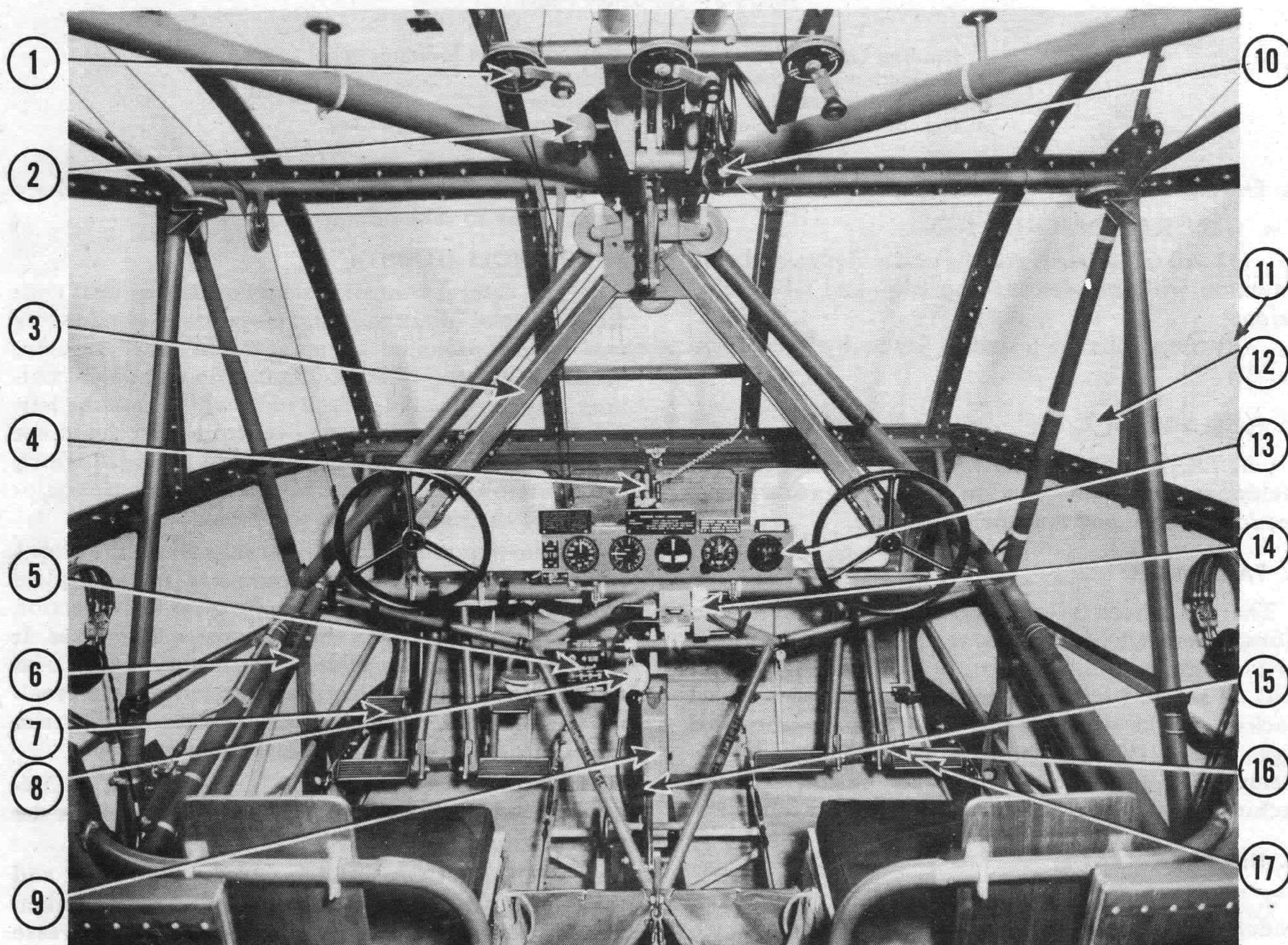
Figure 2—Cockpit and Flying Controls
