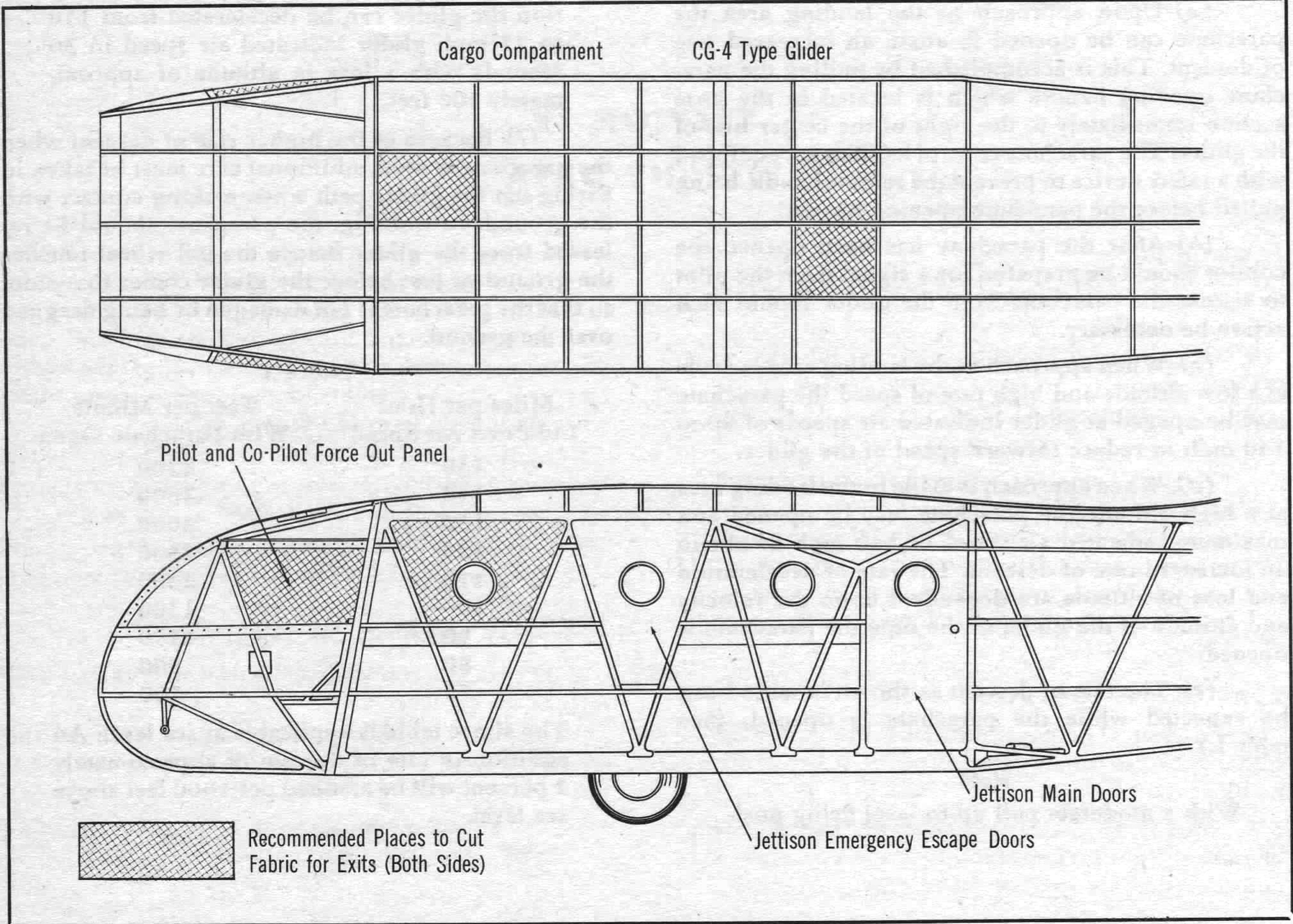
Figure 6—Emergency Exits
