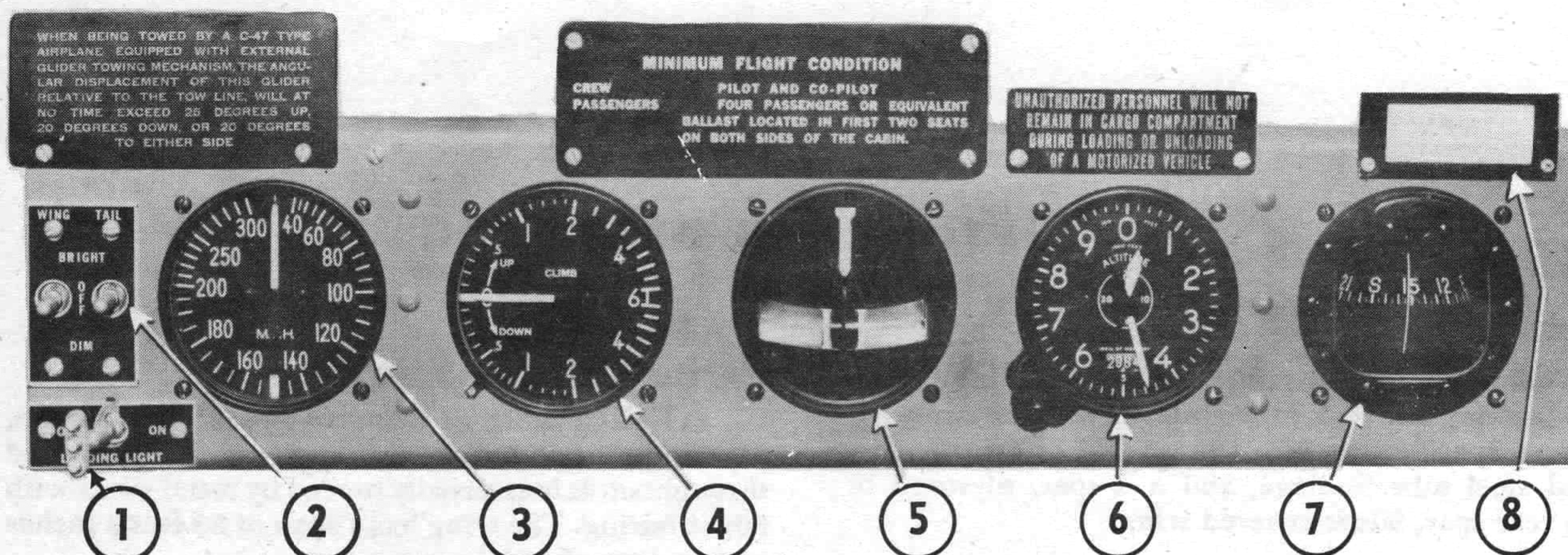
Figure 3—Instrument Panel
