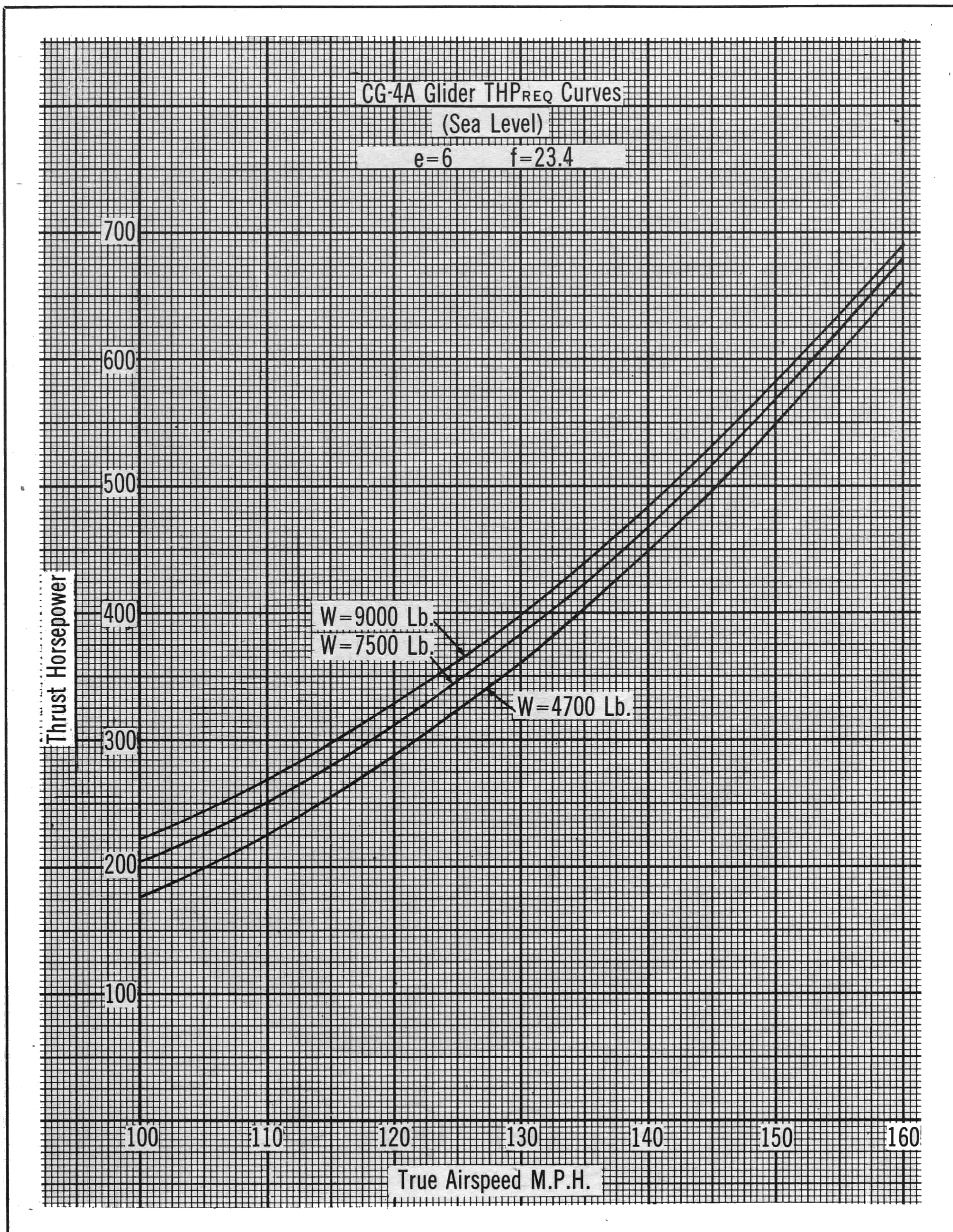
Figure 9—Power Required Curve
