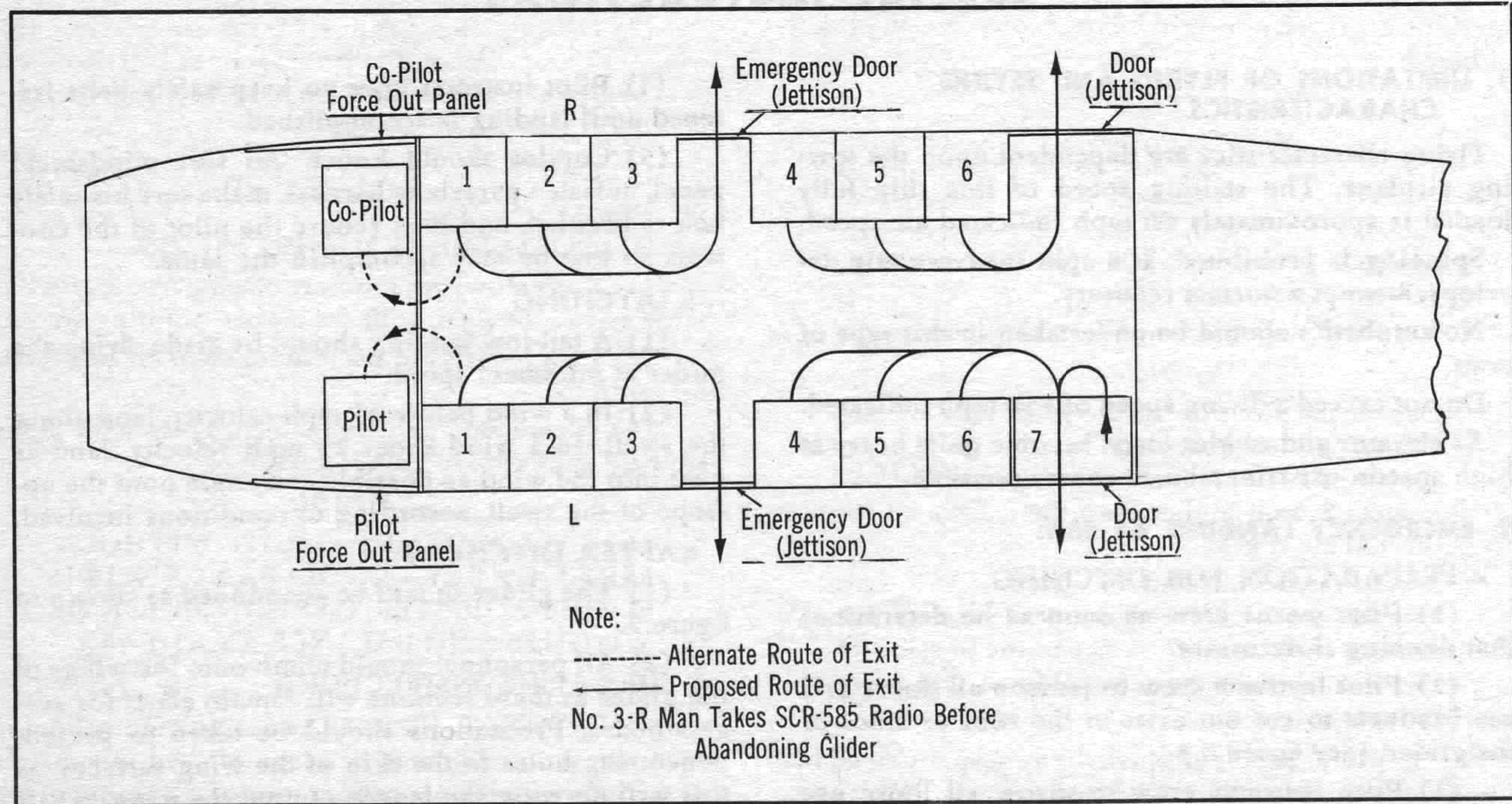
Figure 7—Method of Abandoning CG-4A Glider
