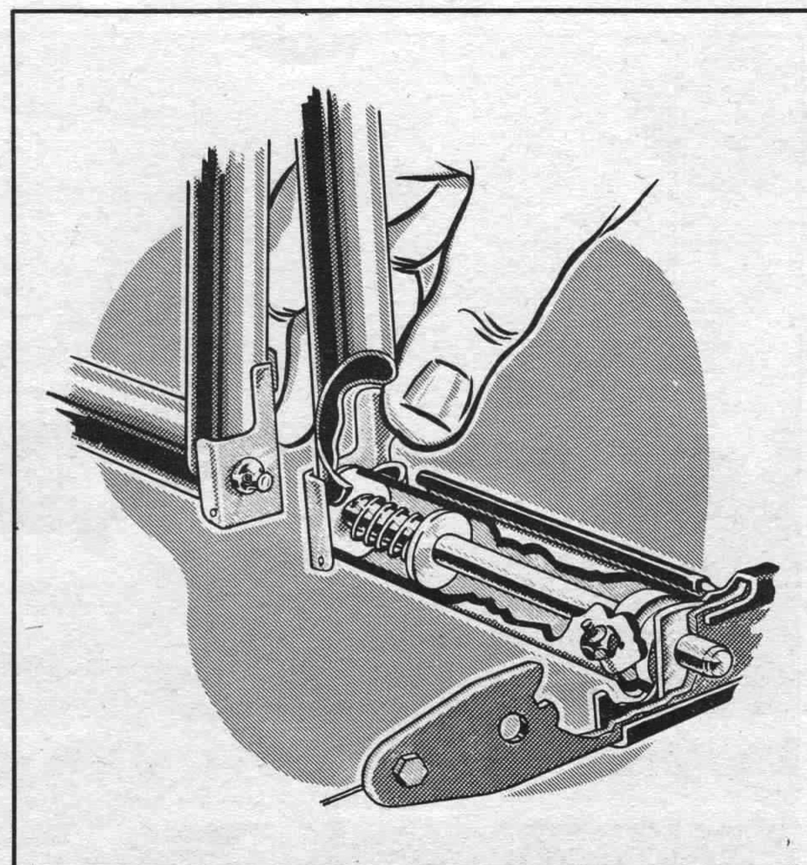
Figure 4—Pedal Adjustment
